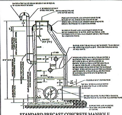
STANDARD PRECAST CONCRETE MANHOLE WITH EXTENDED MONOLITHIC BASE
