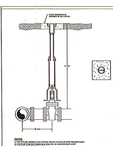
TOWN OF FRONT ROYAL STANDARD WATER DETAILS
