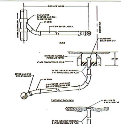
BY PVC CLEANOUT ASSEMBLY. 2-4" BENCH, RISER, AND FLOOD
