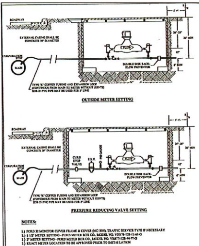
TOWN OF FRONT ROYAL STANDARD WATER DETAILS
