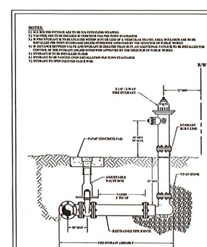
TOWN OF FRONT ROYAL W-13
