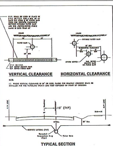
TOWN OF FRONT ROYAL STANDARD WATER DETAILS STANDARD CLEARANCES
