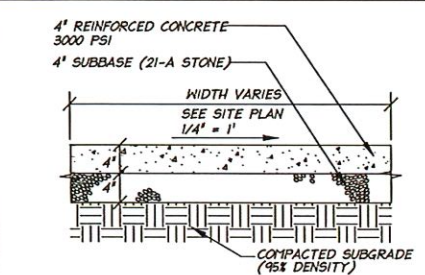
CONCRETE SIDEWALK DET
