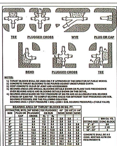
TOWN OF FRONT ROYAL STANDARD WATER DETAILS HORIZONTAL THRUST BLOCK
