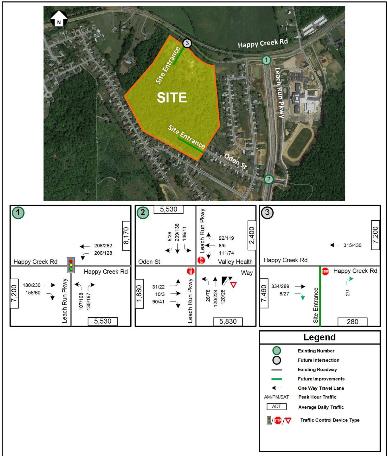
Figure 14: 2028 Future Conditions with Development
