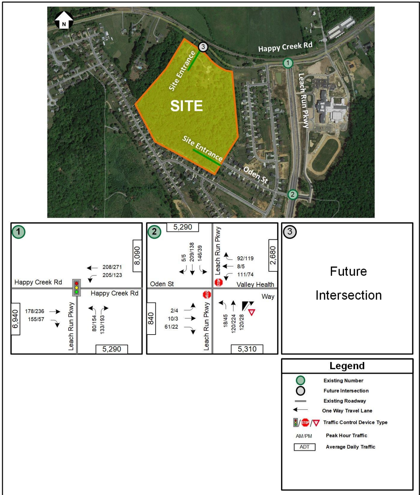
Figure 9: 2028 Future Conditions without Development – Vehicular Traffic Volumes
