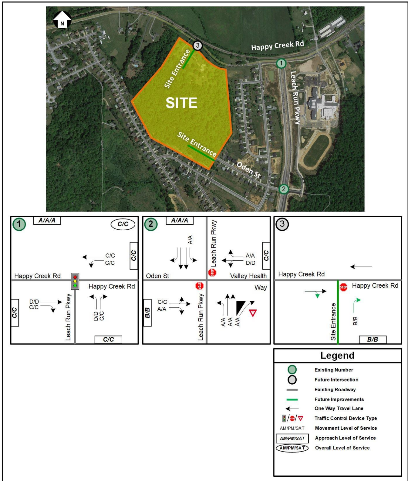
Figure 15: 2028 Future Conditions with Development – Level of Service Results
