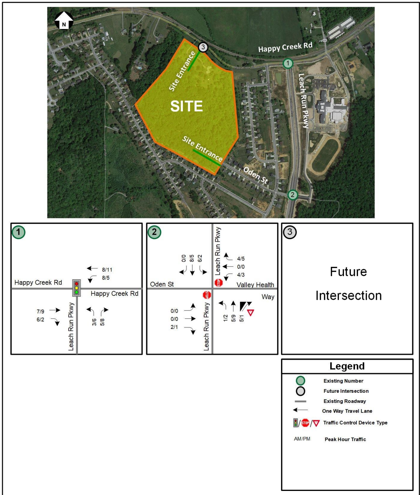
Figure 8: Projected Inherent Regional Growth Traffic Volumes (2024 to 2028)
