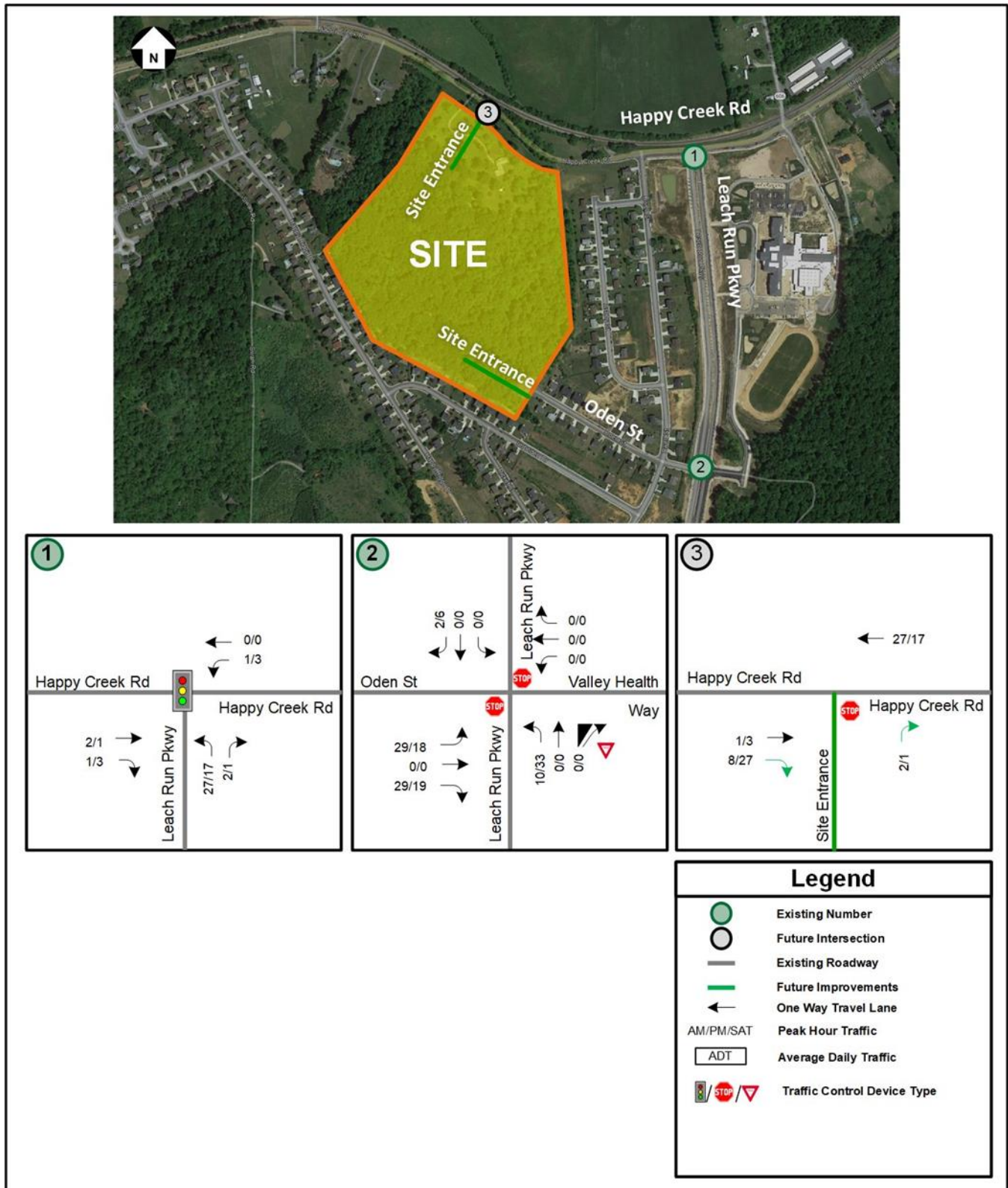
Figure 13: Site Generated Trip Assignment
