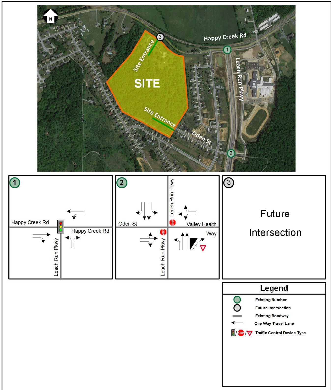
Figure 5: 2024 Existing Conditions – Roadway Network Geometric Configuration and Traffic Control Devices
