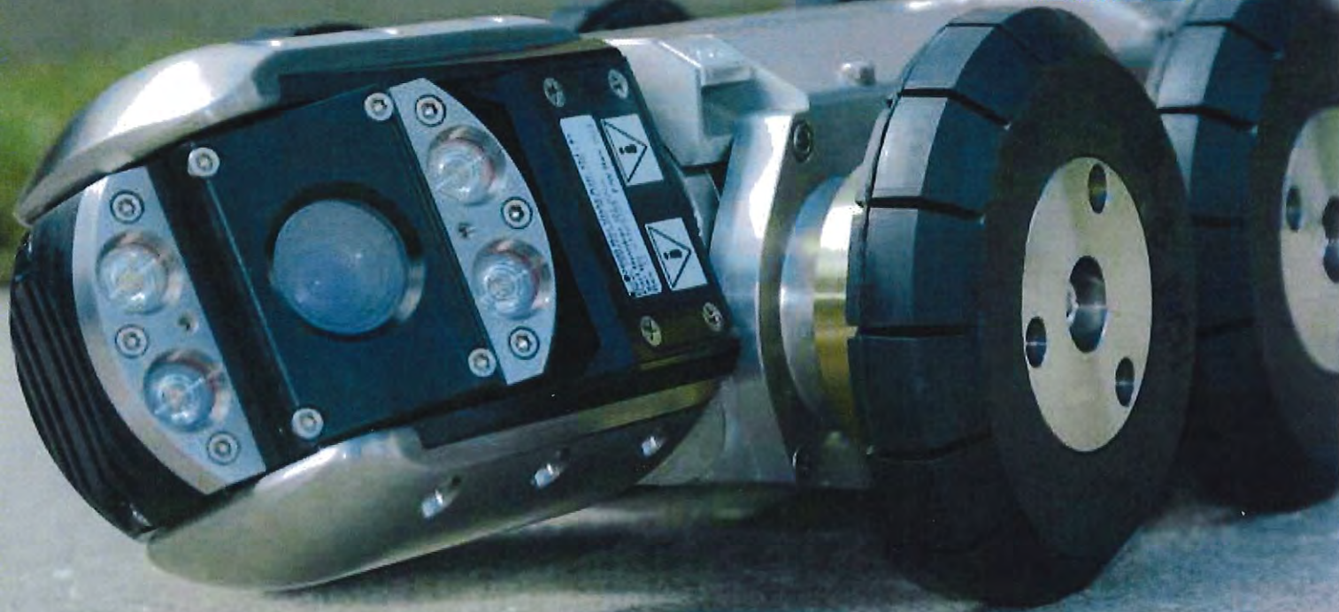
OZIII Camera shown on the optional CUES CPR transporter.
